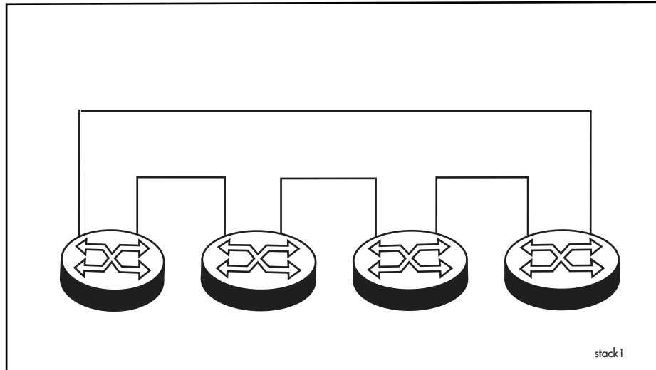
Figure 2-1: Ring Topology
