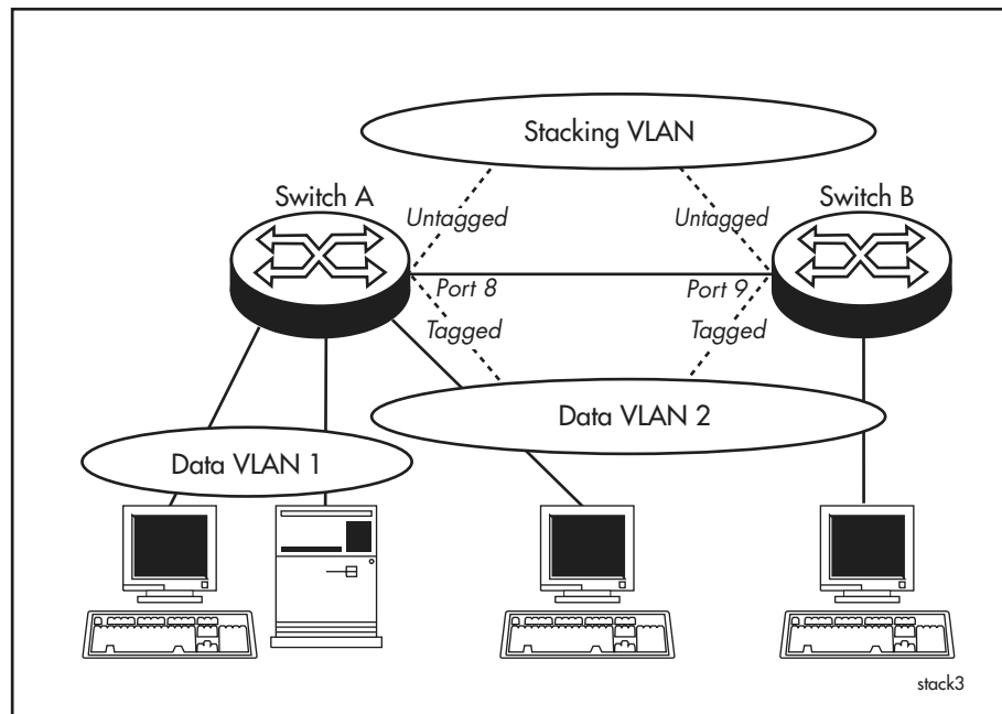
Figure 2-3: VLAN Ports for Stacking
