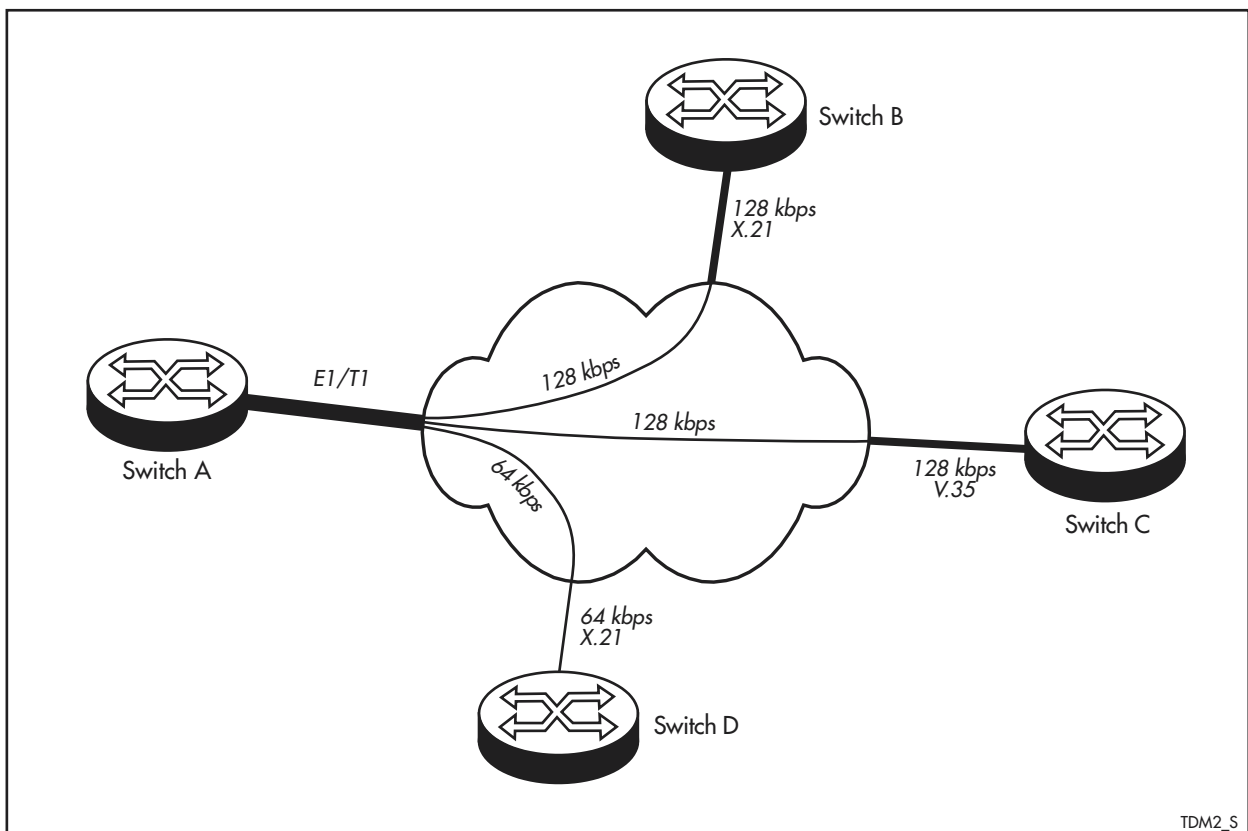
Figure 30-2: A TDM star network.
