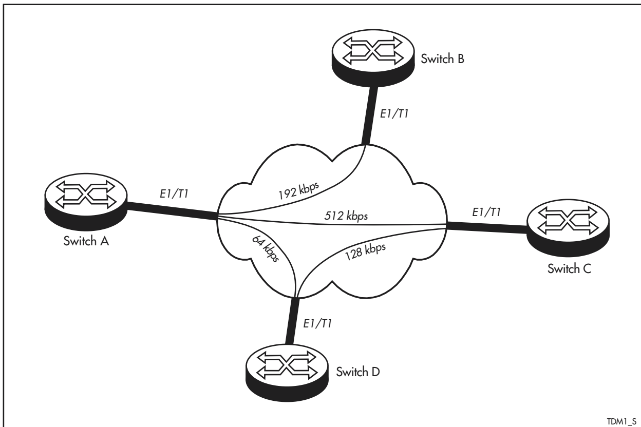
Figure 30-1: Illustration of an E1/T1 network.
