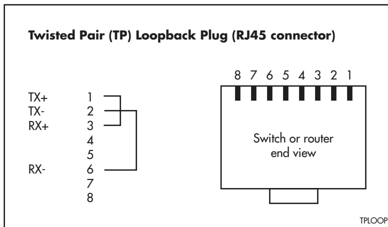
Figure 30: Ethernet twisted pair (TP) loopback plug.
