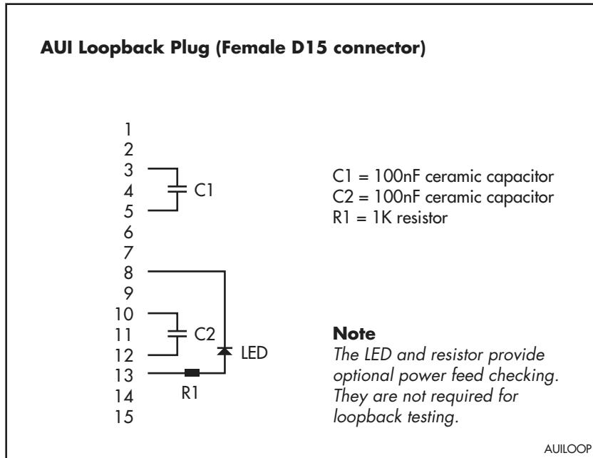
Figure 29: Ethernet AUI loopback plug.
