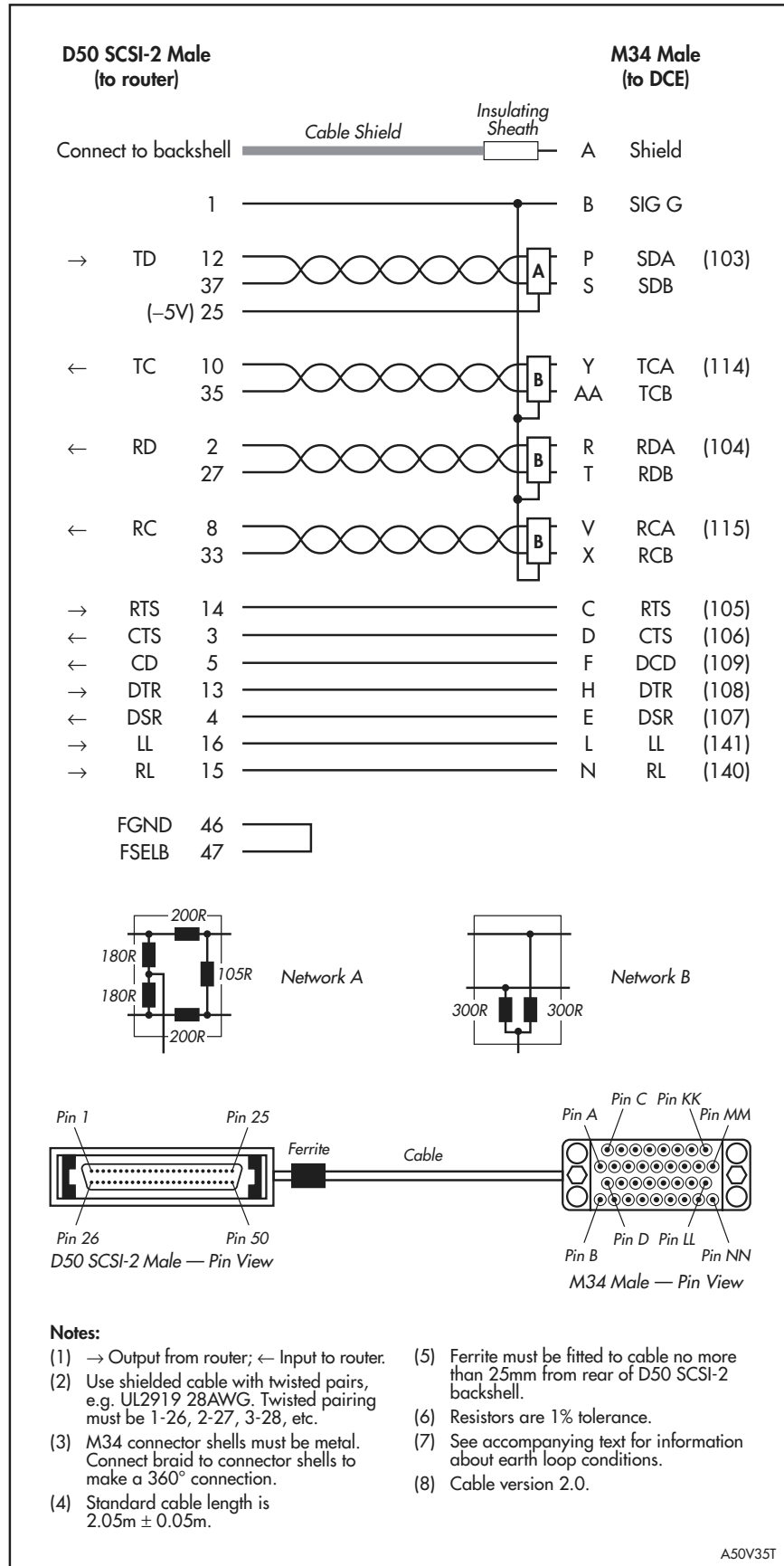
Figure 18: Pin wiring diagram for a V.35 DTE transition cable to an AMPLIMITE 50-way connector.
