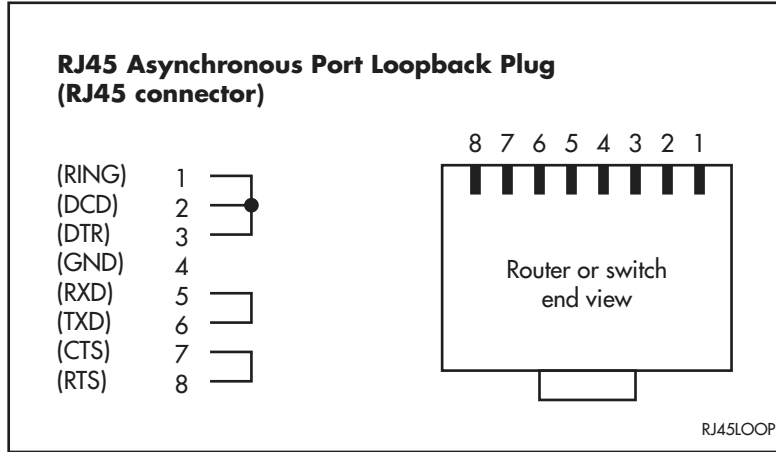
Figure 28: RJ-45 loopback plug for testing asynchronous interfaces.
