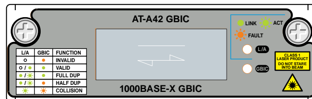
Figure 8: AT-A42-X (GBIC) Uplink Module.
