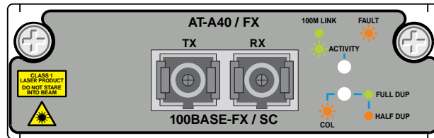
Figure 4: AT-A40-FX (SC) Uplink module.
